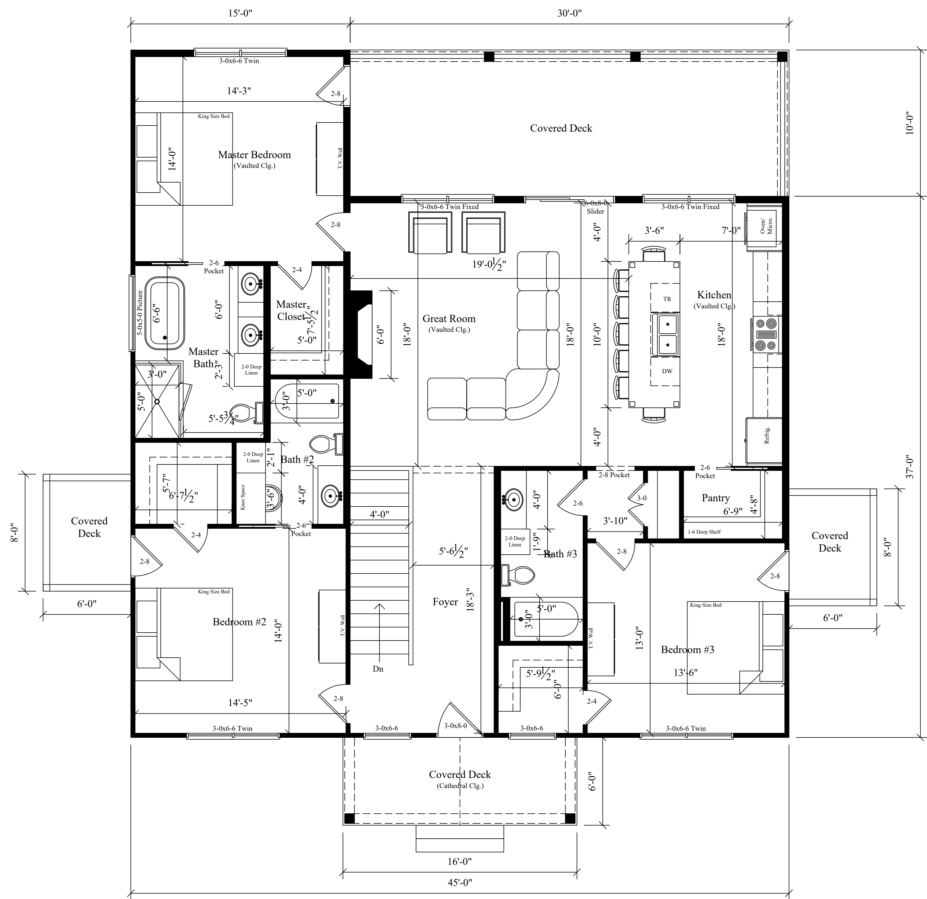
MAIN FLOOR PLAN 1,815 Conditioned Sq.Ft.
