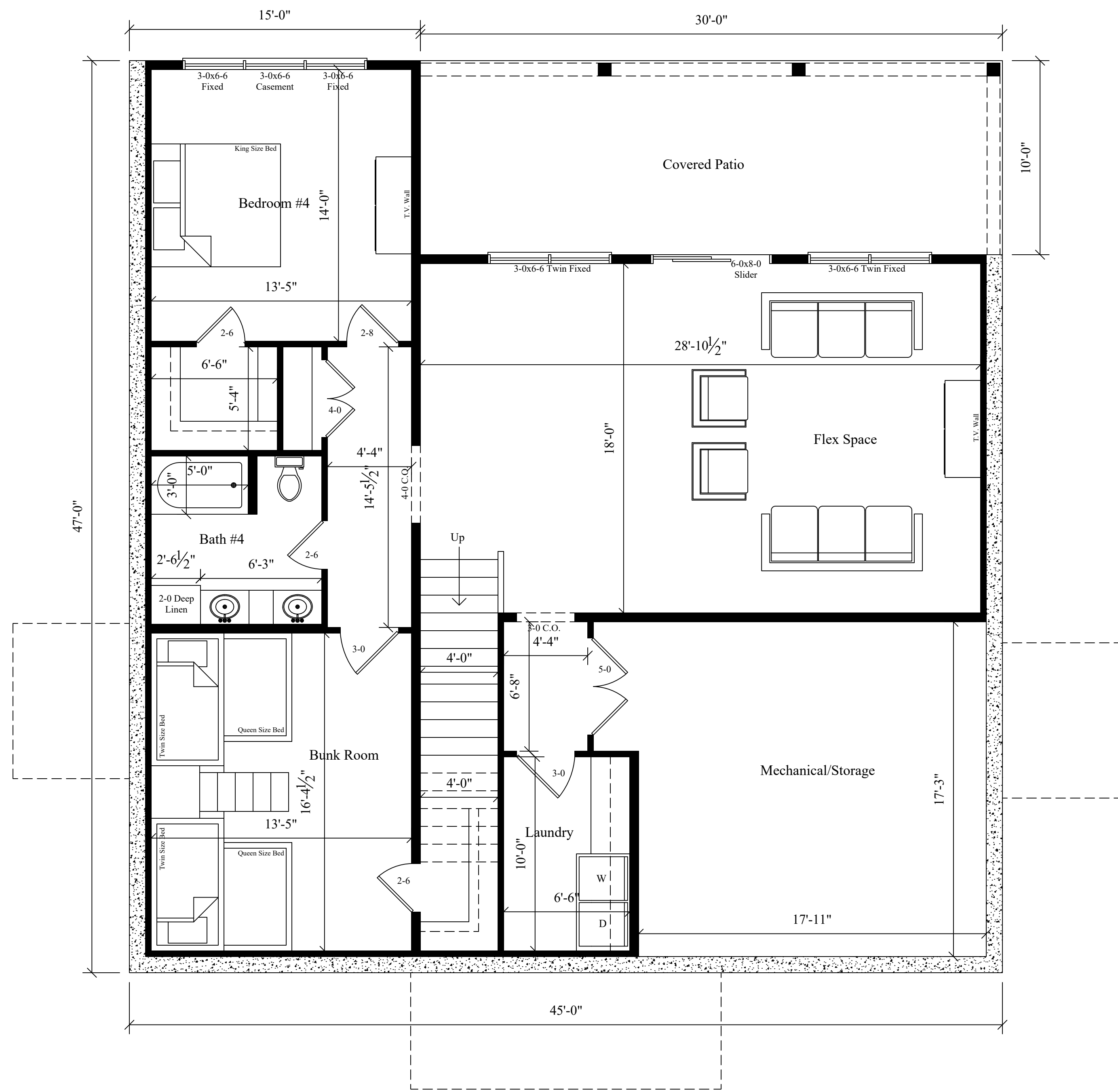
BASEMENT FLOOR PLAN 1,815 Conditioned Sq.Ft.
