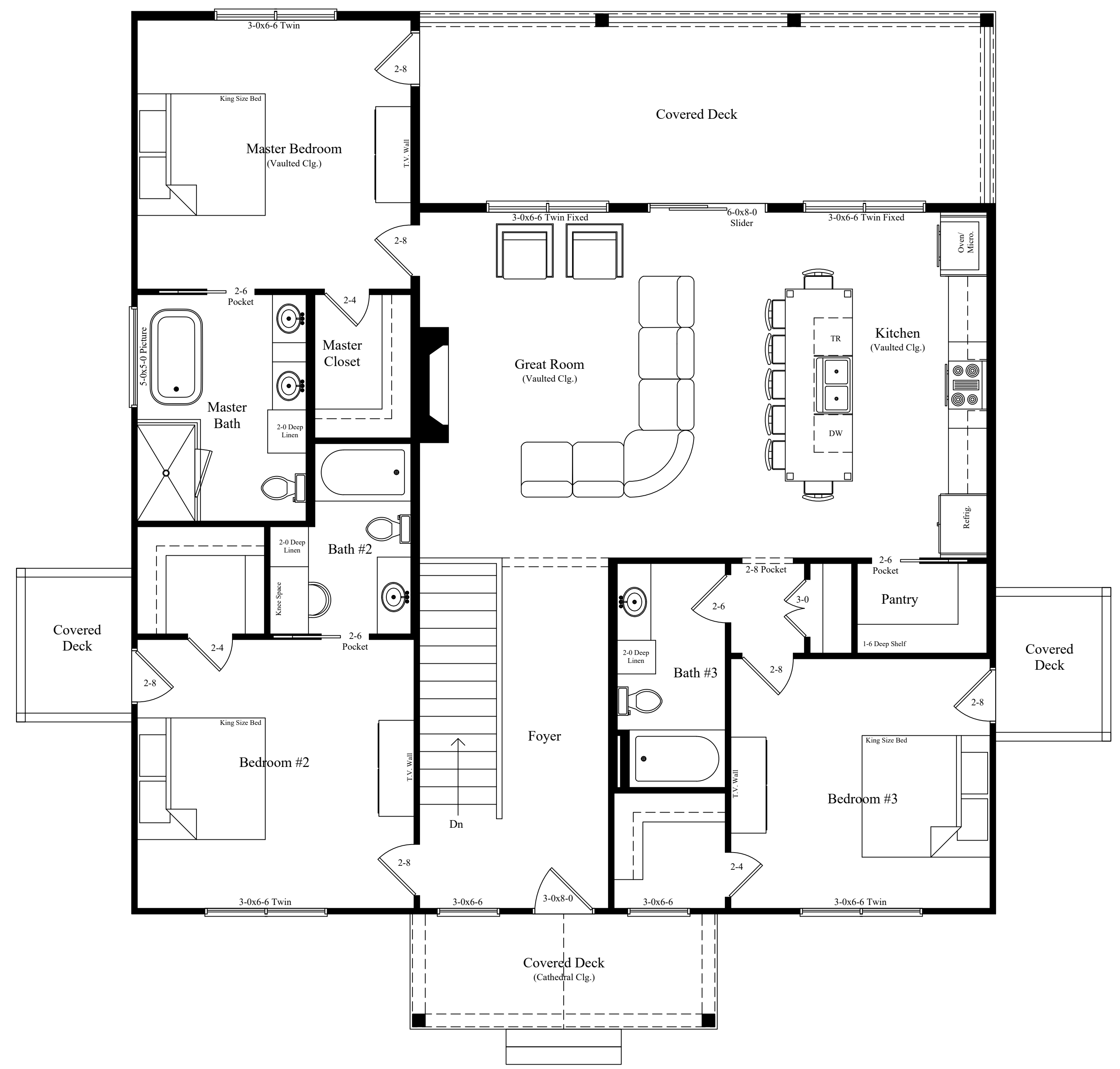
MAIN FLOOR PLAN 1,815 Conditioned Sq.Ft.
